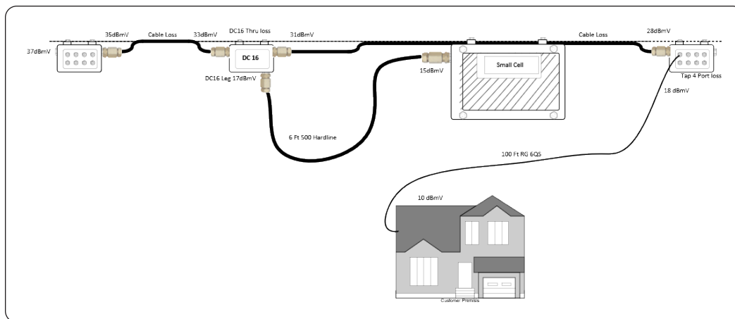
Figure 15 – Directional Couplers for Small Cells
