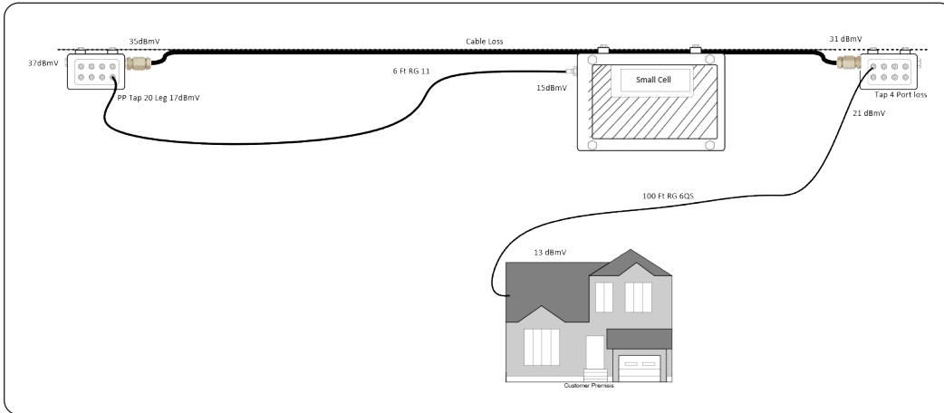
Figure 16 – Power Passing Taps for Small Cells
