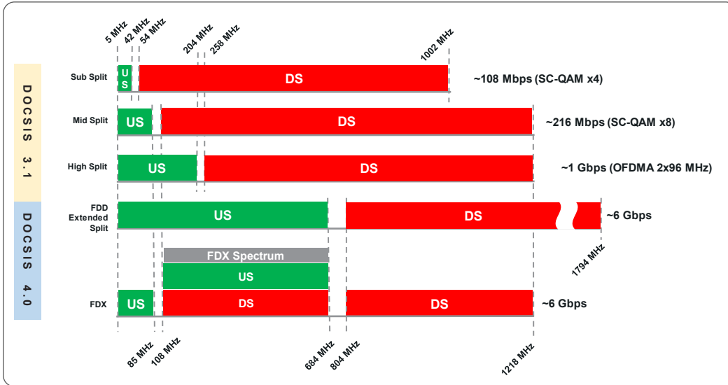
Figure 14 – DOCSIS - Diplex Splits & Upstream Data Limits
