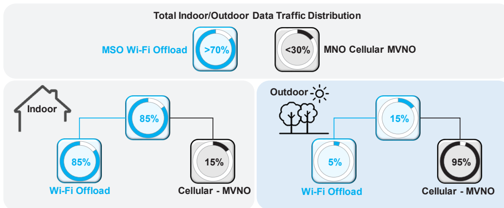
Figure 1 - MVNO Offload Distribution – Wi-Fi Offload Only
