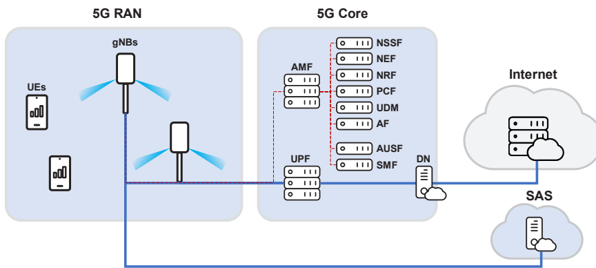
Figure 5 – 5G CBRS Network Architecture
