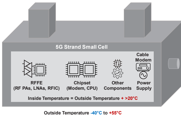
Figure 12 – Strand Small Cell Heat and Loading
