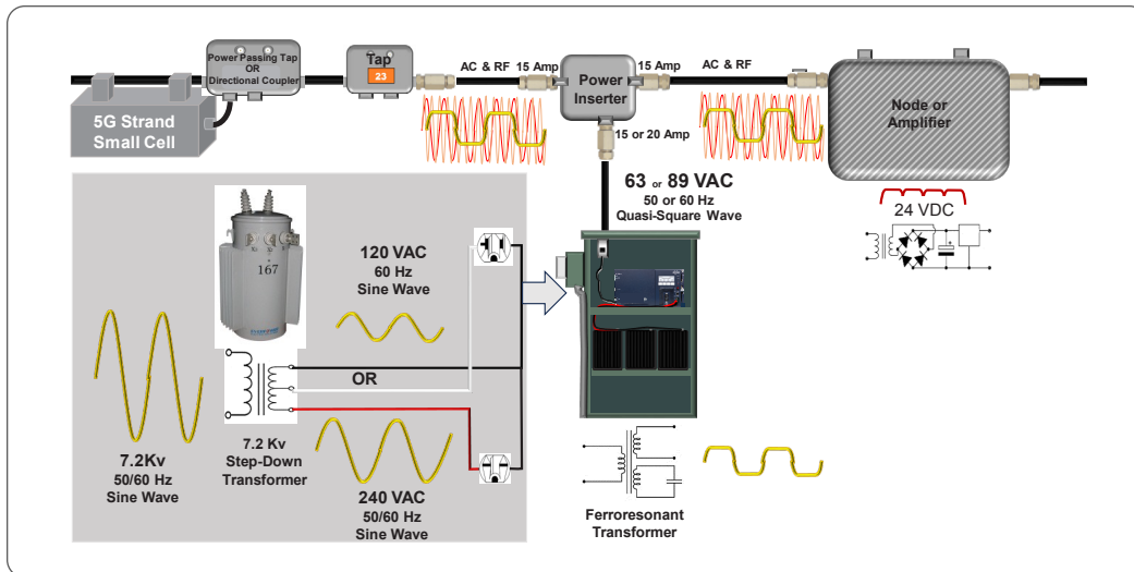
Figure 13 – Broadband Network Power - Overview
