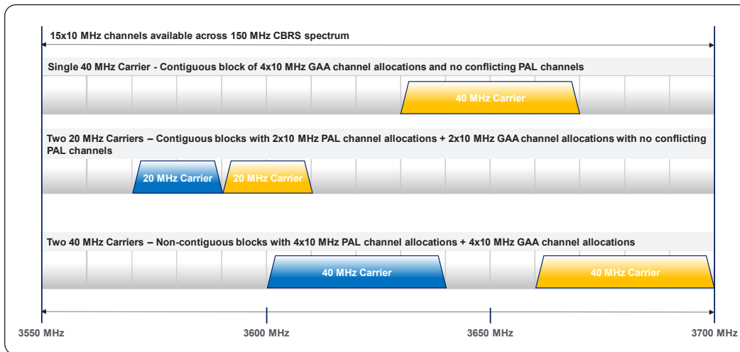
Figure 8 – CBRS Channel Bandwidth, Component Carriers, and Carrier Aggregation
