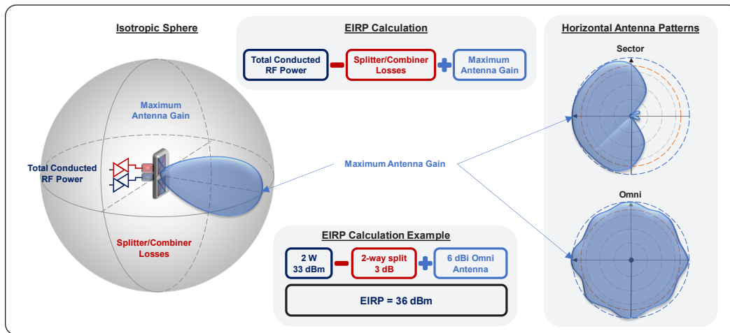
Figure 21 – Effective Isotropic Radiated Power Concept
