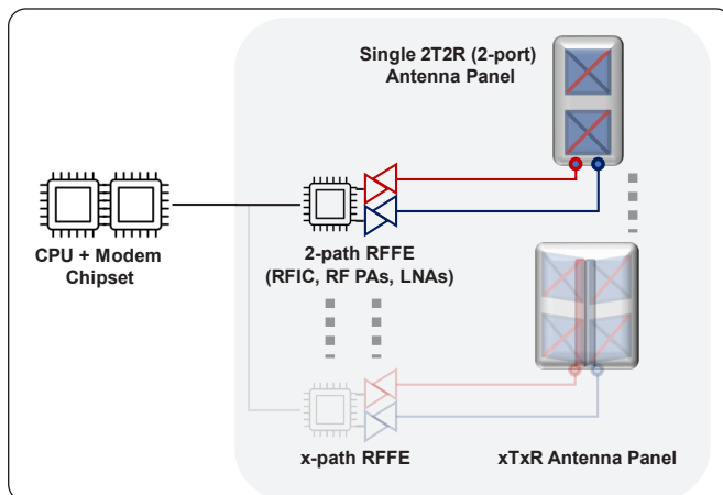
Figure 20 – xTxR Small Cell RF Chain
