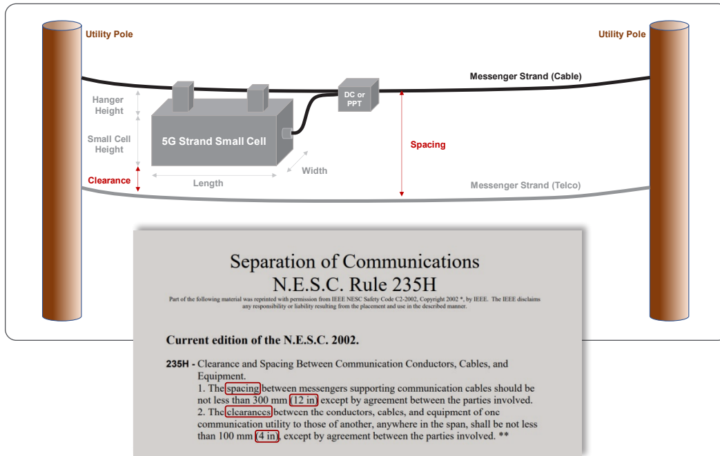
Figure 9 – Strand Small Cell Dimensions and Cable Clearance
