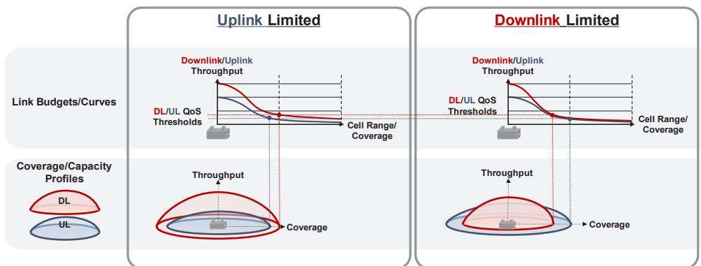
Figure 23 – Wireless Coverage and Capacity
