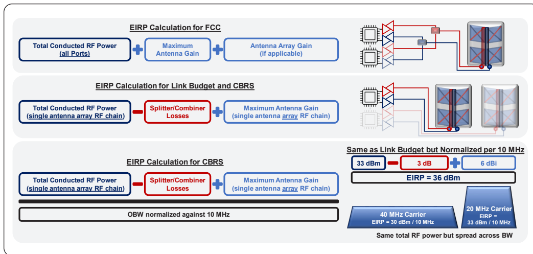
Figure 22 – EIRP Calculation Comparison – FCC, Link Budget, and CBRS
