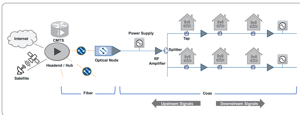
Figure 3 – HFC Network Architecture
