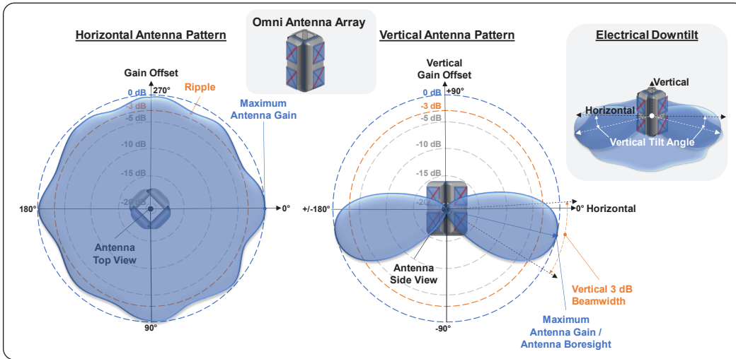
Figure 18 – Electrical Characteristics - Omni Antenna Array
