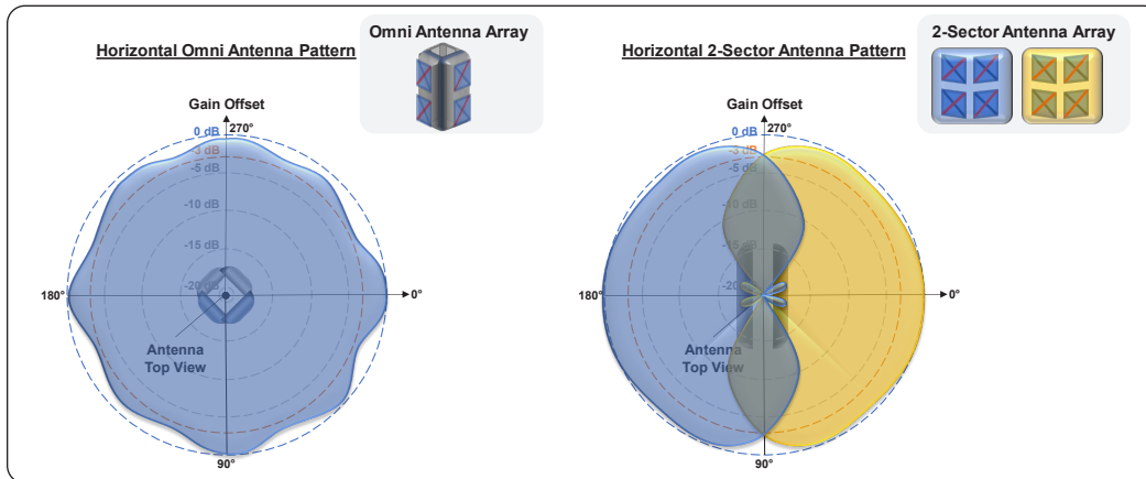
Figure 17 – Wireless Antenna – Omni and Sector
