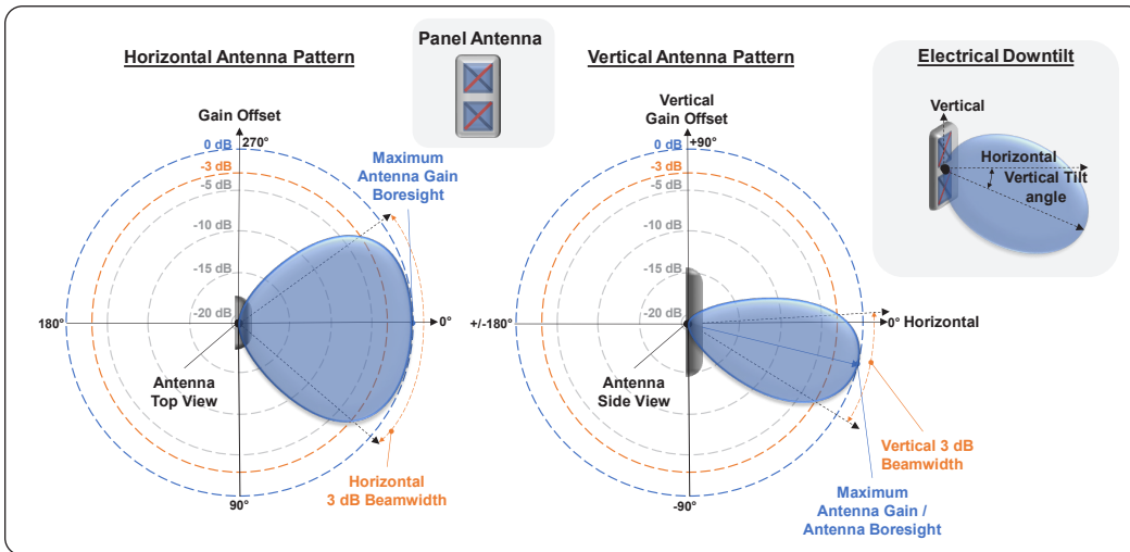
Figure 19 – Electrical Characteristics - Sector / Panel Antenna
