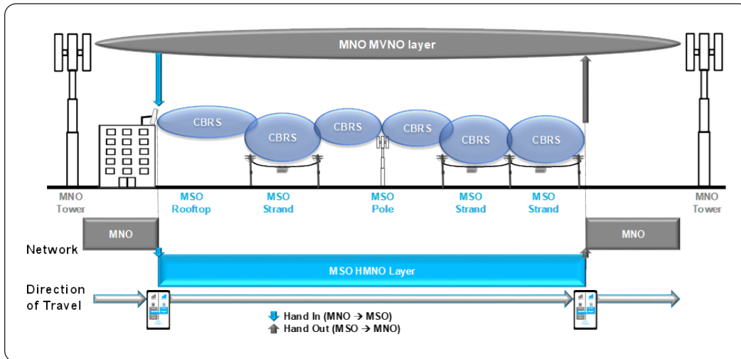
Figure 24 – MNO to MSO MVNO Data Offload – Mobility
