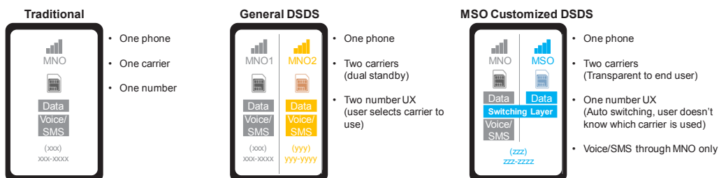
Figure 6 – MNO to MSO MVNO Data Offload – DSDDS
