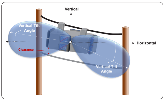
Figure 11 – Mechanical Tilt - Omni Strand Antenna
