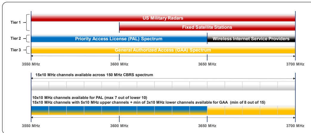
Figure 7 – CBRS Wireless Spectrum
